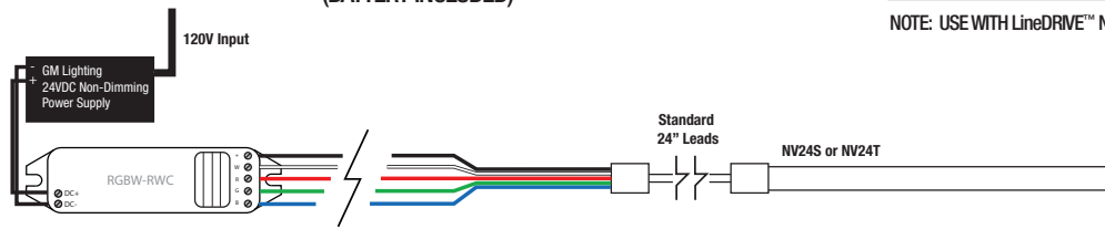
RGBW-RWC CONTROLLER AND REMOTE (BATTERY INCLUDED)
